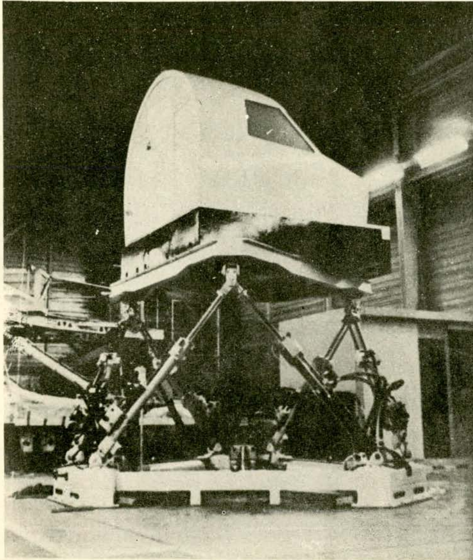
Training Simulator
