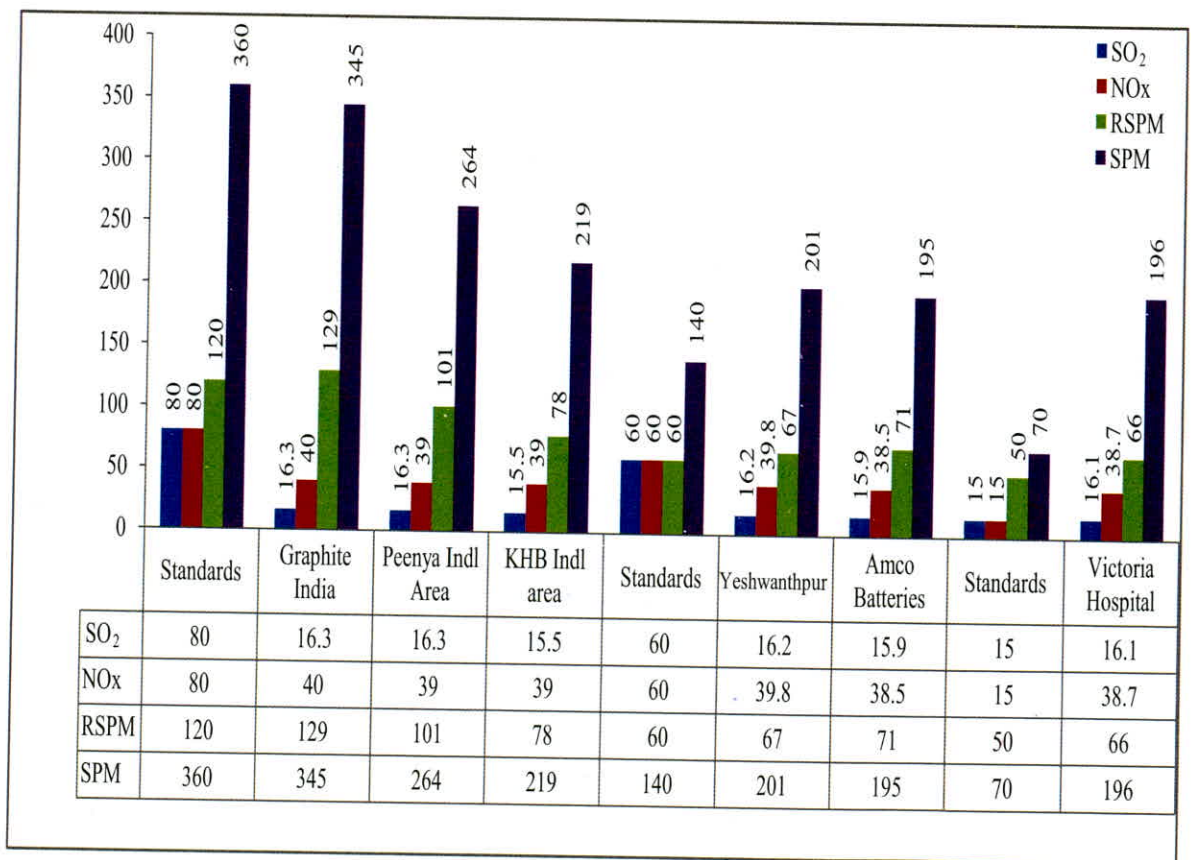
Annual average values of air pollutants at different locations in Bangalore city for the year 2007-08
