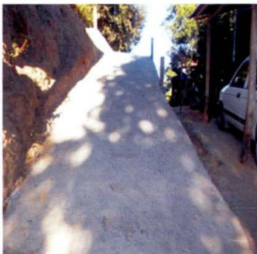
A photograph showing Construction of Stone Masonry steps with masonry pavement alongwith hand railing near Chawngkunga garage to Nunzami house, Luangmual (no hand railing provided)
